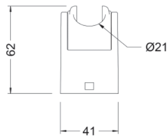
Ref.: 1000 67 45 Soporte ducha GE2 GE2 shower holder
