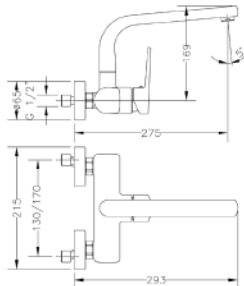
Ref.: 64192 16 45 66 Monomando de fregadera mural Wall single lever sink mixer
