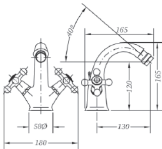
Ref.: 68516 09 43 66 Monobloc bidet bronce Bronze bidet mixer
