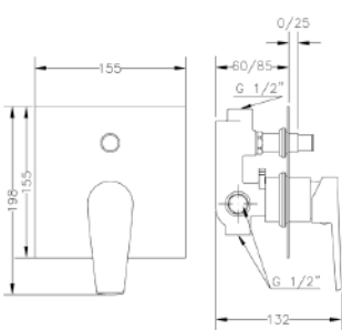
Ref.: 64116 16 45 66 Monomando de baño empotrado con inversor Built-in single lever bath mixer with diverter
