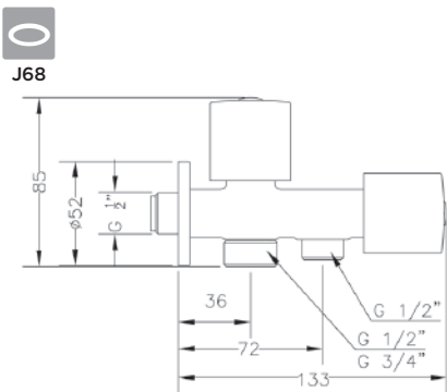
Ref.: 1023 04 Grifo doble combinable 1/2"-3/4" y 1/2" Double outlet tap 1/2"-3/4" and 1/2"
