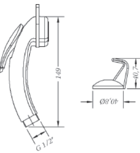
Ref.: 100696 45 Kit ducha sanitaria Sanitary shower kit Box: 1 | Carton: 100 | Pallet: 1800
