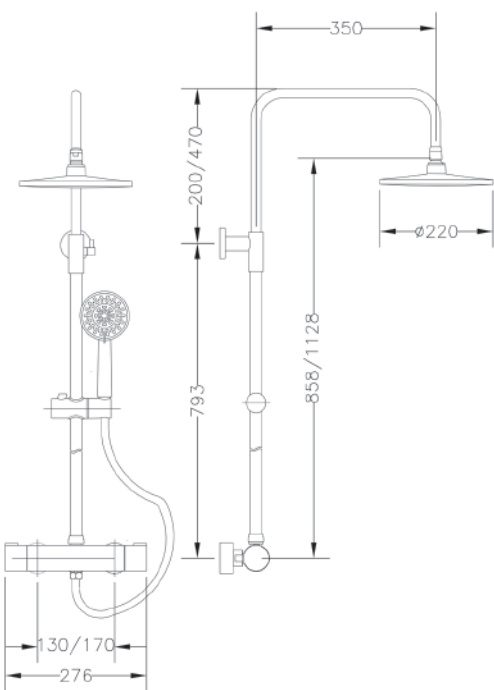
Ref.: CT67110 18 Columna termostática extensible con kit Thermostatic extensible column with kit
