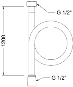
Ref.: 100141 45 Flexo H 1/2" - H 1/2" 1,20 m inoxidable F 1/2" - F 1/2" Stainless steel flexible hose 1.20 m
