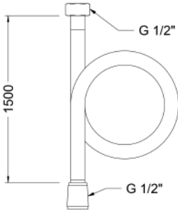
Ref.: 9908 0206 Flexo H 1/2" - H 1/2" 1,5 m cromado F 1/2" - F 1/2" 1.5 m chromed flexible hose
