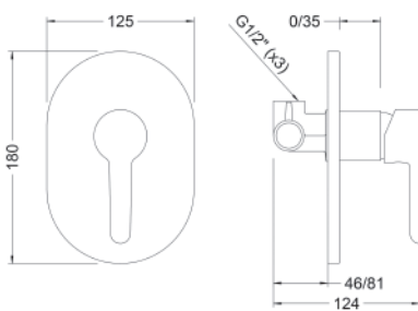
Ref.: 65115 19 45 66 Monomando de ducha empotrado Built-in single lever shower mixer
