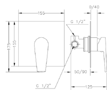
Ref.: 64115 16 45 66 Monomando de ducha empotrado Built-in single lever shower mixer
