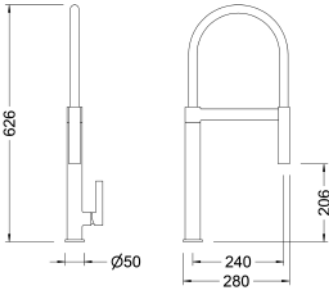
Ref.: 65219 40 60 66 Monomando de fregadera cartucho 25 Single lever sink mixer 25 cartridge
