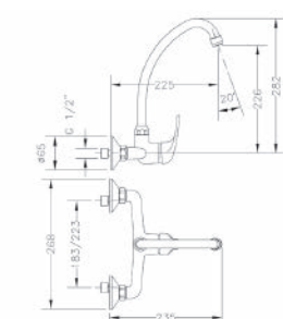
Ref.: 60194 05 45 66 Monomando de fregadera mural 8" Wall single lever 8" sink mixer
