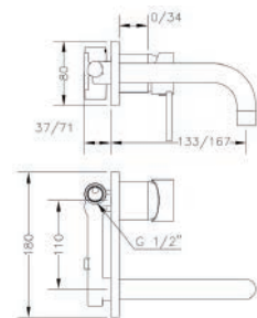
Ref.: 65131 29 45 66 Monomando de lavabo empotrado caño 16 cm Built-in wash-basin mixer 16 cm spout
