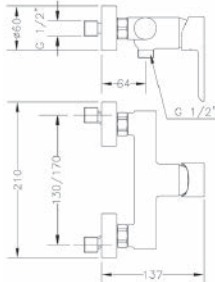
Ref.: 65110 19 45 66 Monomando de ducha con kit Single lever shower mixer with kit
