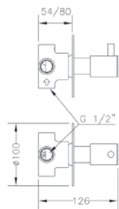
Ref.: 63114 30 45 66 Inversor cerámico 3 vías empotrado placa redonda Built-in 3 way ceramic diverter with round plate Box: 1
