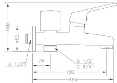
Ref.: 1024 04 Grifo doble combinable a 1/2"- 3/4" y Aireador Double outlet tap 1/2" - 3/4" and aerator
