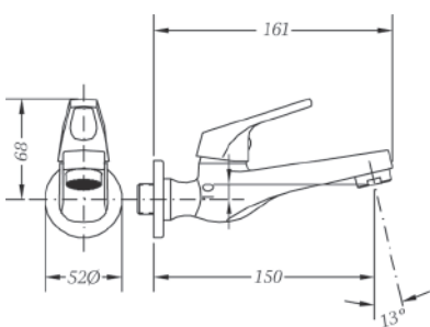
Ref.: 1003 04 Grifo lavabo mural 1 agua cartucho 25 One-water wall wash-basin tap 25 cartridge
