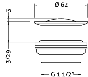
Ref.: 100208 45 Válvula click 1 1/4" bañera 1 1/4" bath click valve
