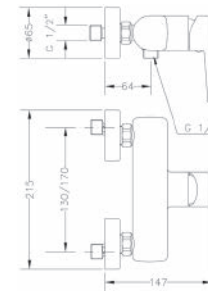
Ref.: 64110 16 45 66 Monomando de ducha con kit Single lever shower mixer with kit
