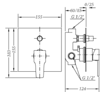
Ref.: 63116 26 45 66 Monomando de baño empotrado con inversor Built-in single lever bath with mixer with diverter
