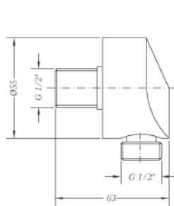
Ref.: 1680 04 Toma ducha mural redonda Round wall flexible connector
