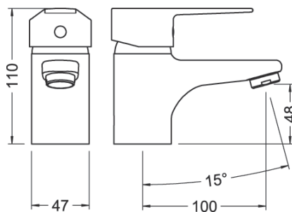
Ref.: 60130 28 45 66 Monomando de lavabo Single lever wash-basin mixer
