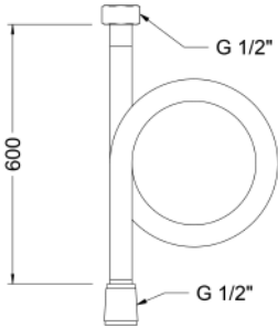
Ref.: 9908 0203 Flexo H1/2" - H1/2" 60cm F1/2"-F1/2" 60cm Flexible hose
