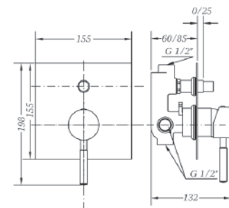
Ref.: 65116 18 45 66 Monomando de baño empotrado con inversor Built-in single lever mixer bath with diverter
