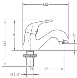
Ref.: 1007 04 Grifo lavabo 1 agua cartucho 25 One-water wash-basin tap 25 cartridge
