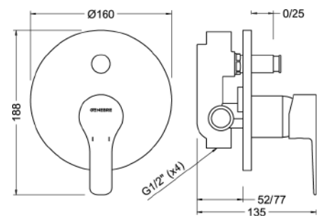
Ref.: 61116 28 45 66 Monomando de baño empotrado con inversor Built-in single lever bath mixer with diverter
