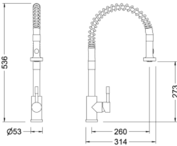
Ref.: 65207 18 60 66 Monomando de fregadera inox con muelle y ducha extraíble Stainless steel single lever sink mixer with spring and pull-out sprayer
