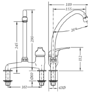
Ref.: 60199 05 45 66 Monomando mesada 6" 6" widespread single lever sink mixer
