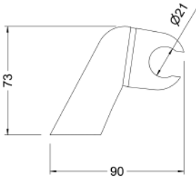
Ref.: 100152 45 00 Soporte ducha Combi Combi shower holder
