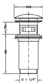
Ref.: 100210 45 Válvula click 1 1/4" con/sin rebosadero 1 1/4" click valve with/out overflow
