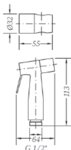
Ref.: 100694 45 Kit ducha sanitaria Sanitary shower kit Box: 1 | Carton: 22 | Pallet: 268
