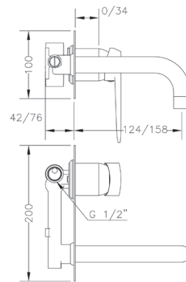
Ref.: 62131 31 45 66 Monomando de lavabo empotrado caño 16 cm Built-in wash-basin mixer 16 cm spout
