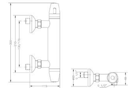
Ref.: 67104 14 45 67 Termostática ducha Thermostatic shower mixer
