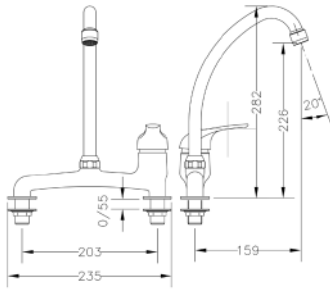
Ref.: 60198 05 45 66 Monomando mesada 8" 8" widespread single lever sink mixer
