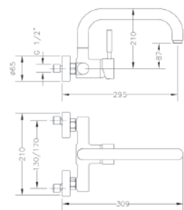
Ref.: 65192 18 45 66 Monomando de fregadera mural 15 cm Wall single lever sink mixer 15 cm
