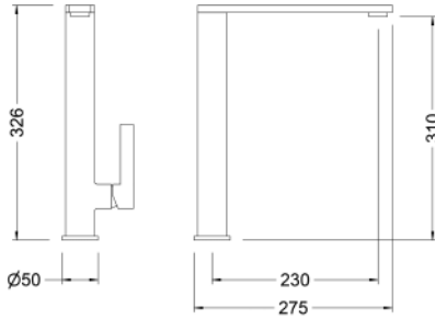
Ref.: 65215 40 60 66 Monomando de fregadera cartucho 25 Single lever sink mixer 25 cartridge
