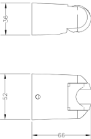
Ref.: 100068 45 Soporte ducha ovalado Oval shower holder
