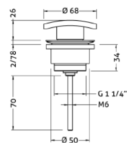
Ref.: 100204 45 Válvula click Kenjo 1 1/4" 1 1/4" Kenjo click valve
