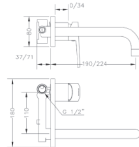
Ref.: 64132 16 45 66 Monomando de lavabo empotrado caño 22 cm Built-in wash-basin mixer 22 cm spout
