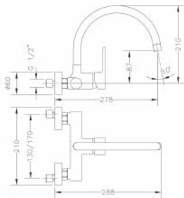
Ref.: 65192 19 45 66 Monomando de fregadera mural 15 cm Wall single lever sink mixer 15 cm
