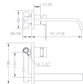
Ref.: 63132 26 45 66 Monomando de lavabo empotrado caño 22 cm Built-in wash-basin mixer 22 cm spout
