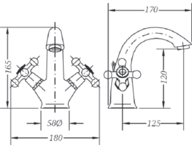
Ref.: 68506 09 43 66 Monobloc de lavabo bronce Wash-basin mixer bronze
