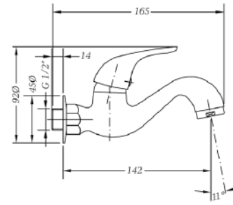
Ref.: 1006 04 Grifo lavabo mural 1 agua cartucho 25 One-water wall wash-basin tap 25 cartridge
