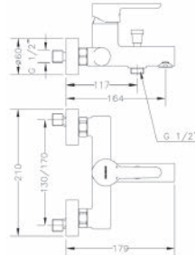
Ref.: 65100 19 45 66 Monomando de baño con kit Single lever bath mixer with kit
