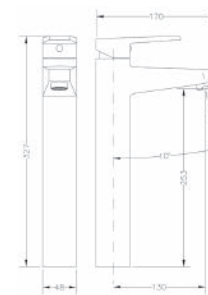
Ref.: 64136 16 45 66 Monomando de lavabo alto High single lever wash-basin mixer
