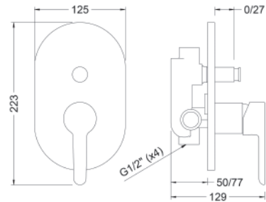
Ref.: 65116 19 45 66 Monomando de baño empotrado con inversor Built-in single lever bath mixer with diverter
