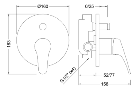
Ref.: 61116 22 45 66 Monomando de baño empotrado con inversor Built-in single lever bath mixer with diverter
