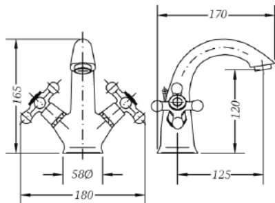
Ref.: 68506 09 45 66 Monobloc de lavabo cromo Chromed wash-basin mixer
