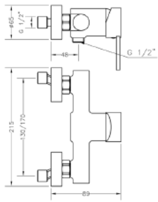
Ref.: 65110 29 45 66 Monomando de ducha con kit Single lever shower mixer with kit
