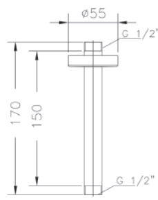
Ref.: 1671 45 Brazo a techo redondo 15 cm Round roof arm 15 cm Box: 1 | Carton: 20 | Pallet: 600
