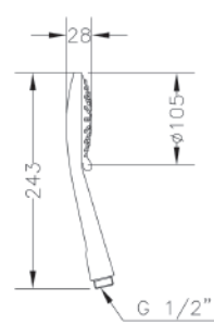
Ref.: DXT3 45 Mango de ducha T3 jets T3 jets handshower
