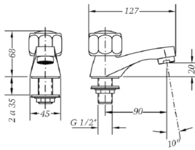
Ref.: 68180 11 45 66 Grifo de lavabo Wash-basin tap
