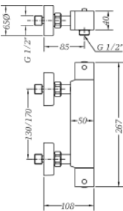
Ref.: 67110 26 45 67 Termostática ducha sin kit Thermostatic shower mixer without kit
