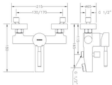
Ref.: 65100 18 45 66 Monomando de baño con kit Single lever bath mixer with kit
