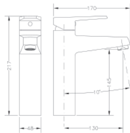
Ref.: 64134 16 45 66 Monomando de lavabo medio alto Medium height single lever wash-basin mixer
