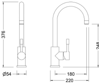
Ref.: 65203 18 60 66 Monomando de fregadera inox caño cisne Stainless steel single lever sink mixer with swan spout
