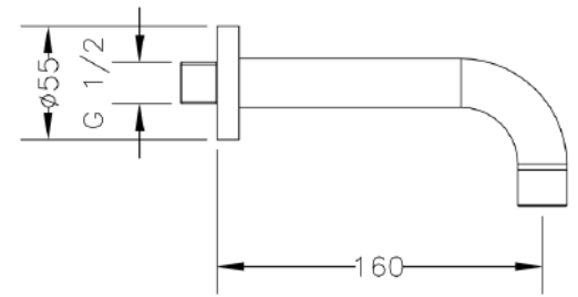
Ref.: 68911 45 Caño mural tubo recto 16 cm Wall mounted pipe spout 16 cm
