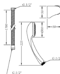
Ref.: 100697 45 Kit de ducha GE2, flexo, soporte y ducha 1 jet GE2 shower set, flexible hose, holder and 1 jet handshower
