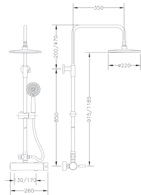
Ref.: CM65110 18 Columna monomando extensible con kit Single lever extensible column with kit
