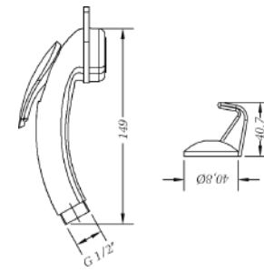
Ref.: 100696 45 Kit ducha sanitaria Sanitary shower kit
