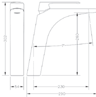
Ref.: 62136 08 45 66 Monomando de lavabo alto High single lever wash-basin mixer
