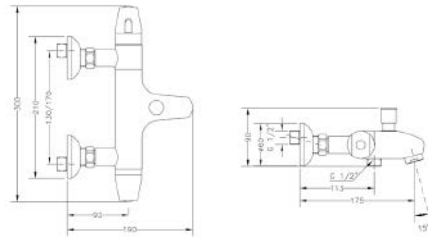
Ref.: 67103 14 45 67 Termostática baño Thermostatic bath mixer
