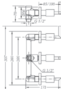
Ref.: 68116 12 45 66 Grupo ducha empotrado 8\"/> Built-in 8" shower mixer with diverter
